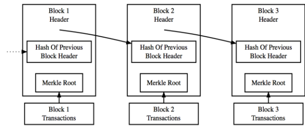
Figure 1. Blockchain Illustration
